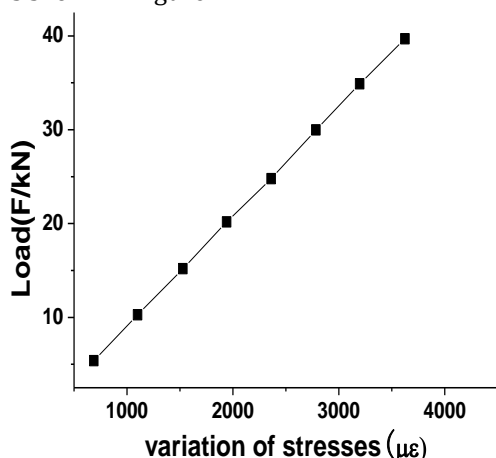
Figure 1: Calibration curve of bolt load
