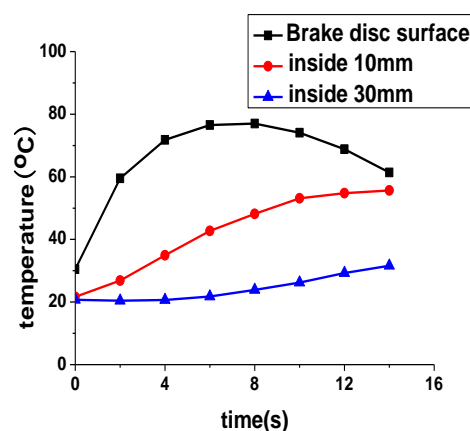
Figure 3: Temperature curve of brake disc at different axial positions with time
