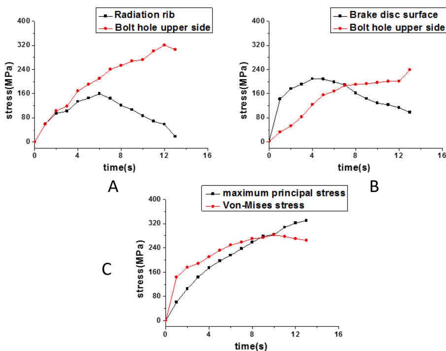
Figure. 5 Stress analysis diagram of finite element model (A. Maximum principal stress on the upper side of radiating rib and bolt hole; B. Von-Mises equivalent stress on friction surface and upper side of bolt hole; C. Relation diagram of Von-Mises stress and maximum principal stress of brake disc with time)
