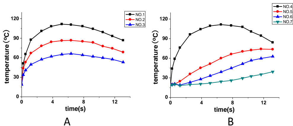
Figure 4: Temperature-time curves at different locations (A. Radial different positions; B. Axial different positions)
